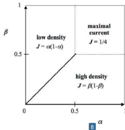
Figure 2. The Phase Diagram of the TASEP, with Open Boundary Conditions and Sequential Updating Dynamics
