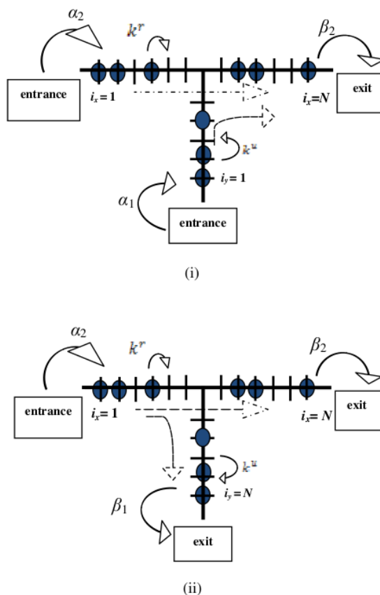
Figure 3. The Dynamics of TASEP in 2D for a Three-way Junction with (i) two Entrances and One Exit, and (ii) One Entrance and Two Exits
