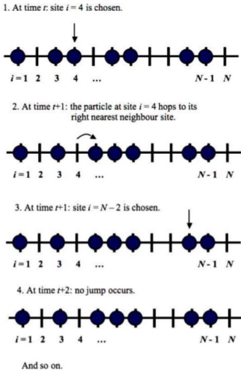
Figure 1. An Example of the Sequential Updating Process of the TASEP (Taken from [12])
