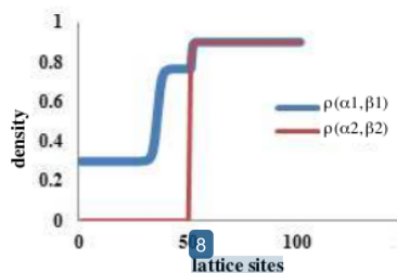
Figure 5. The Density Profile of the TASEP in 2D for a Three-way Junction with One Entrance and Two Exits in the CP-HD Phase. The Horizontal Axis Presents the Lattice Sites from 1 to 100. The Vertical Axis is the Density
